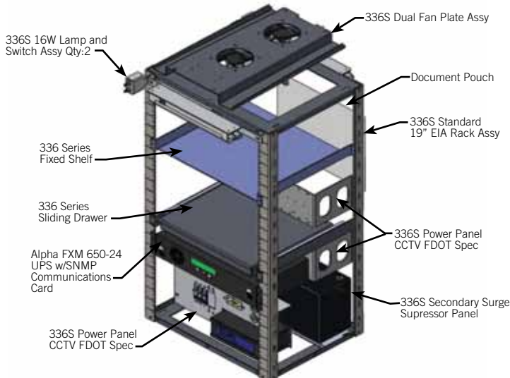
336S Rack for FDOT CCTV with UPS
