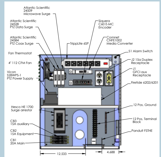
26" x 22" x 18" CCTV Enclosure
